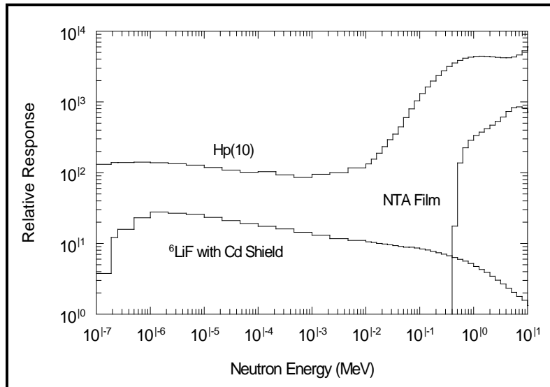
Figure 6.3.2.2-1. Comparison of Hp(10) from normally incident neutrons (IAEA 2001) to the energy responses of a nuclear track type A (NTA) film and a neutron albedo dosimeter containing a neutron thermoluminescent dosimeter (TLND) chip made of lithium-6 fluoride and shielded by cadmium (IAEA 1990, 2001).
