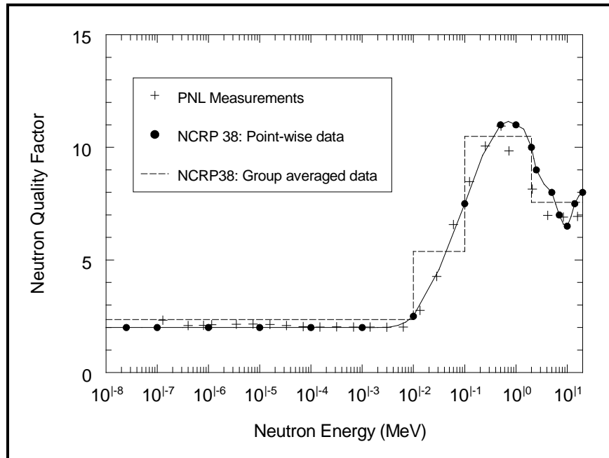
Figure 6.4.2.1-1. Comparison of the neutron quality factors used in the PNL neutron spectrum measurements and the neutron quality factors from NCRP Report 38 (NCRP 1971) shown both as point-wise data and grouped averaged data over the four neutron energy groups used in the dose reconstruction for the Y-12 workers.
