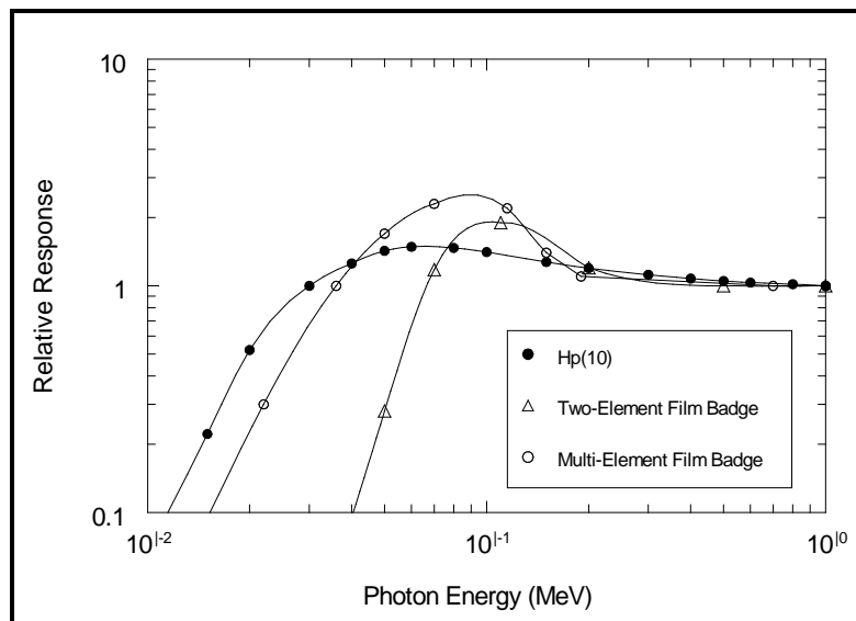
Figure 6.3.2.1-1. Comparison of Hp(10) from a broad beam of normally incident photons (ICRP 1996) with the energy responses for a sensitive DuPont 502 emulsion in a MED two-element film badge (Pardue, Goldstein, and Wollan 1944) and a sensitive DuPont 555 emulsion in an ORNL multi-element film badge (Thornton, Davis, and Gupton 1961).
