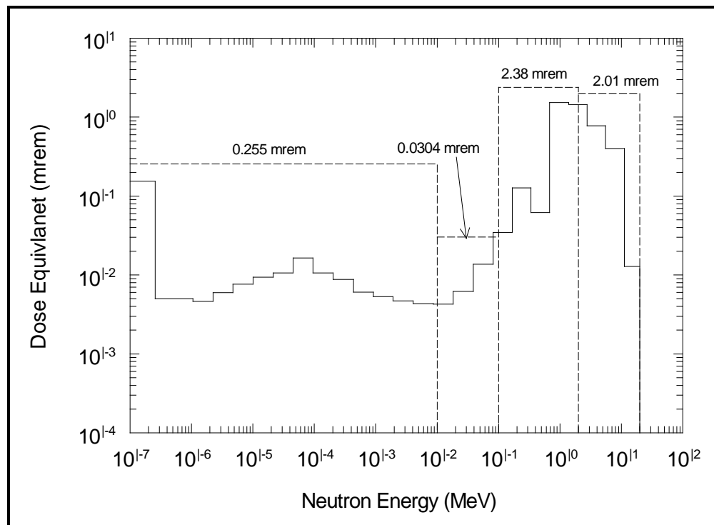
Figure 6.3.4.2-1. Results of PNL neutron spectrum measurements in Calibration Laboratory of Building 9983 are shown by the solid line in the graph and the dashed line shows the PNL measurement results divided into the four neutron energy groups used in the dose reconstruction for the Y-12 workers.
