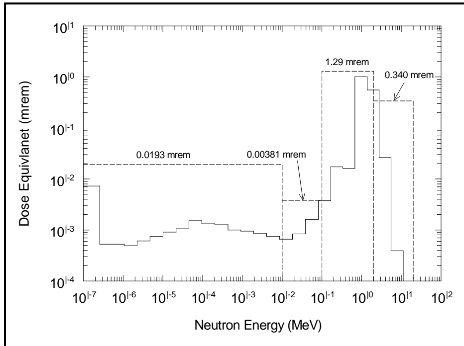
Figure 6.3.4.2-2. Results of PNL neutron spectrum measurements in the Enriched Uranium Storage Area of Building 9212 are shown as the solid line in the graph. The dashed line shows the PNL measurement results divided into the four neutron energy groups used in the dose reconstruction for the Y-12 workers.
