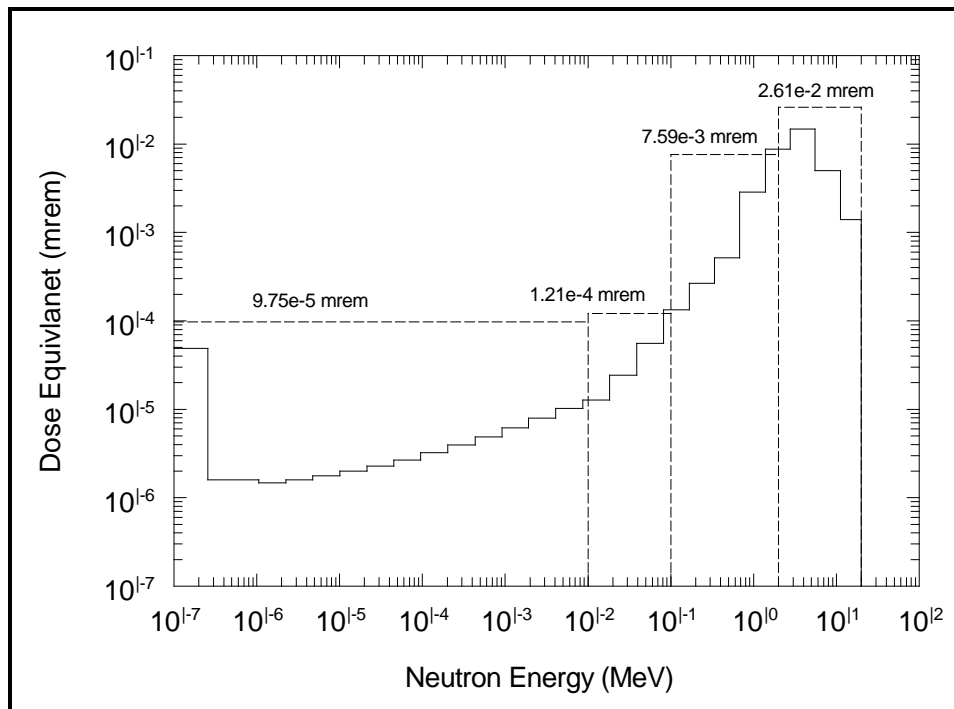
Figure 6.3.4.2-3. Results of PNL neutron spectrum measurements made at 1 meter from a bare ^{252}\text{Cf} fission neutron source are shown by the solid line in the graph and the dash line shows the PNL measurement results divided into the four neutron energy groups used in the dose reconstruction for Y-12 workers at the Nondestructive Analysis Laboratory in Building 9720-5.
