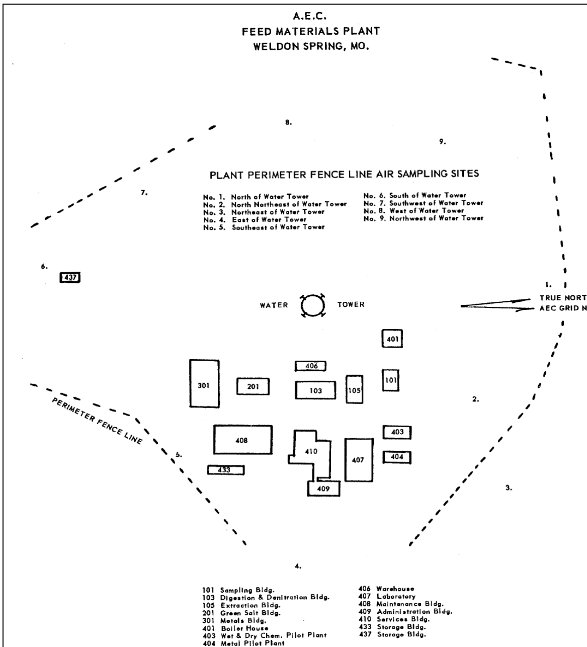
Figure 4-1. Perimeter sampling locations and processing facilities (lacking distance scale) (Meshkov et al. 1986, p. 123).
