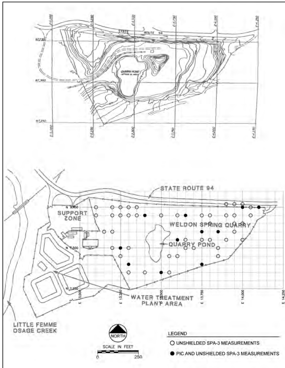
Figure 4-5. Topographic map and locations of gamma exposure rate measurements for WSQ (DOE 1985b, pp. 14, 17).
