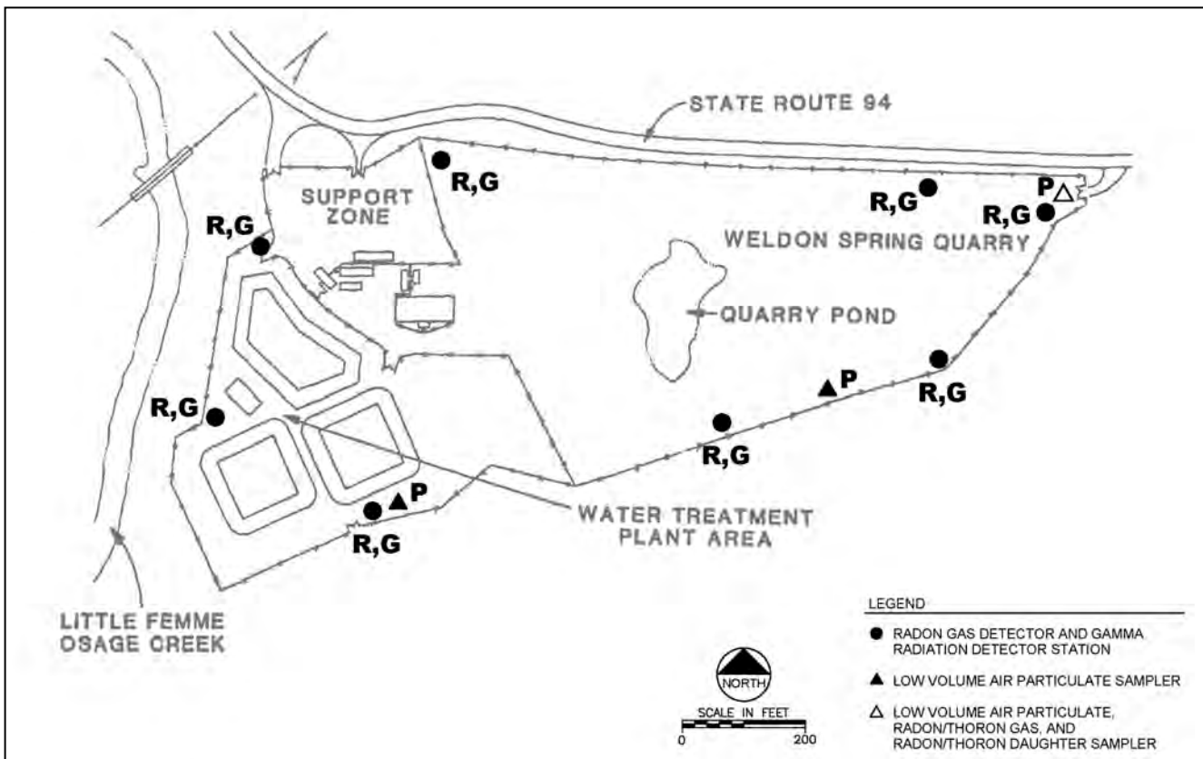
Figure 4-4. Air particulate (P), radon (R), and gamma (G) monitoring stations in WSQ (modified from DOE 1999, p. 70).
