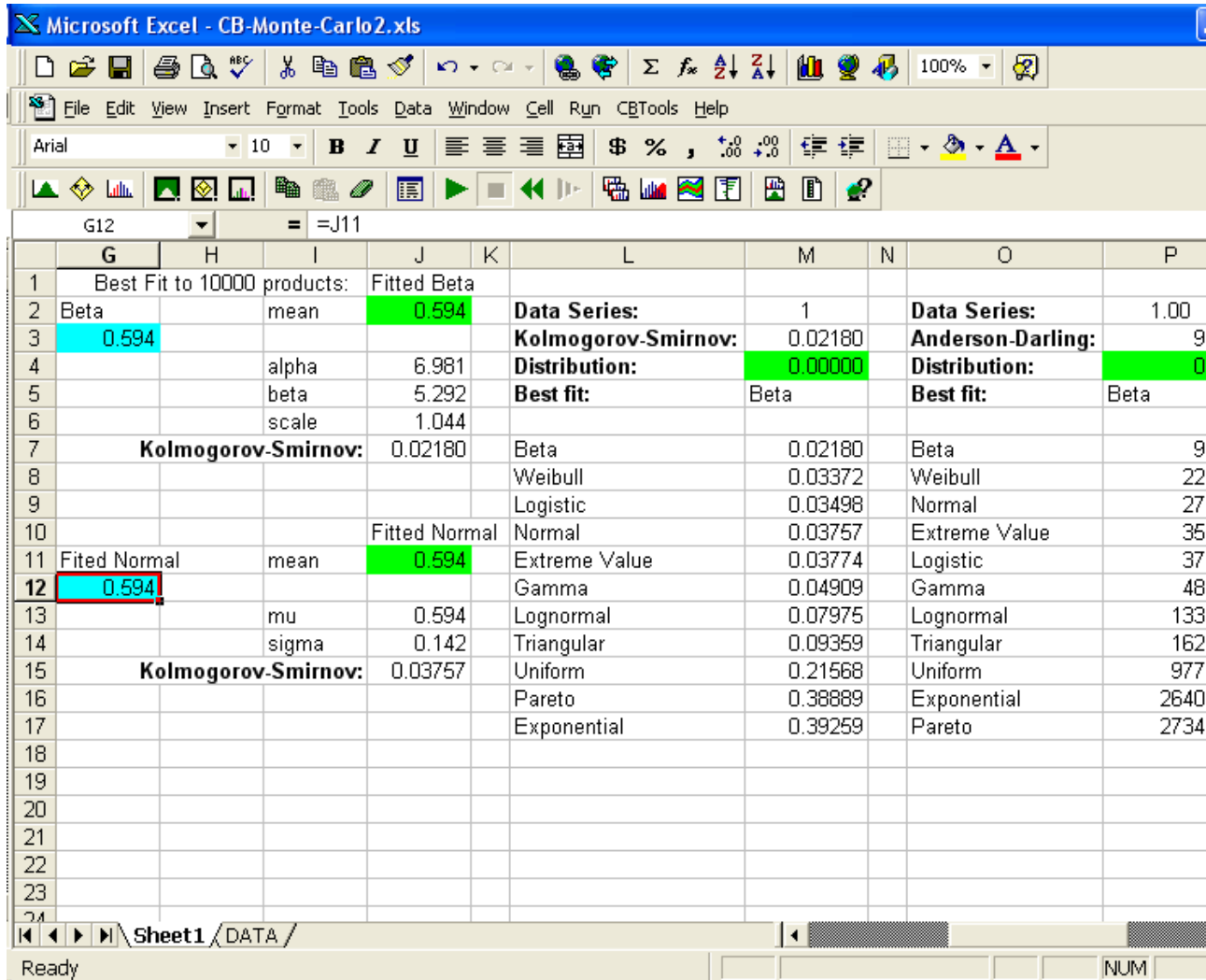
Figure 3.7-1. K-S and A-D Statistics for All Distributions Fitted to a Sample of 10,000 Products using Crystal Ball 2000 Batch Fit Procedure
