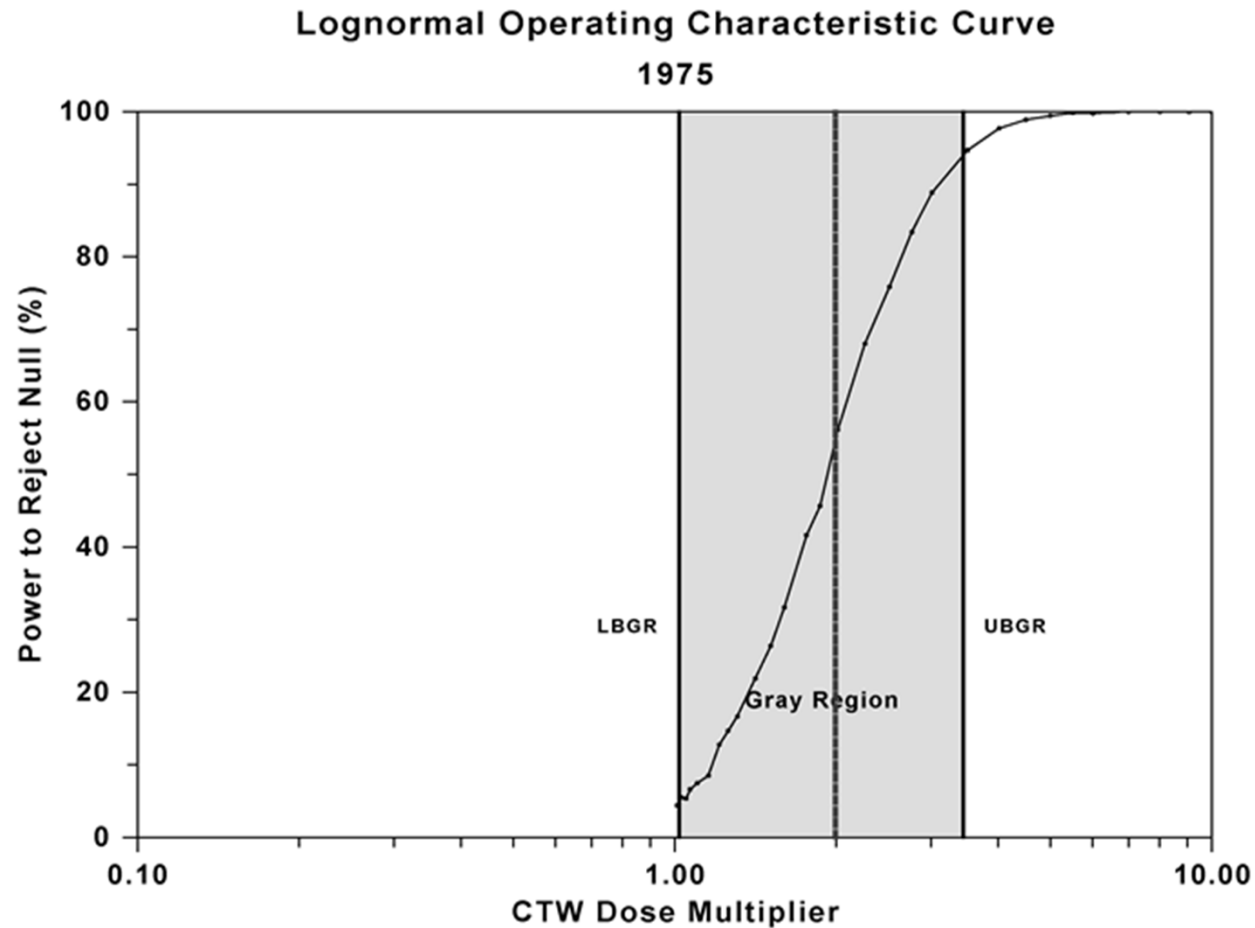
Figure 2. The DQO Process is Used to Define the Gray Region for the Test. Power is Low and Type 2 Error Rates are High Below the Upper Bound of the Gray Region (UBGR)
