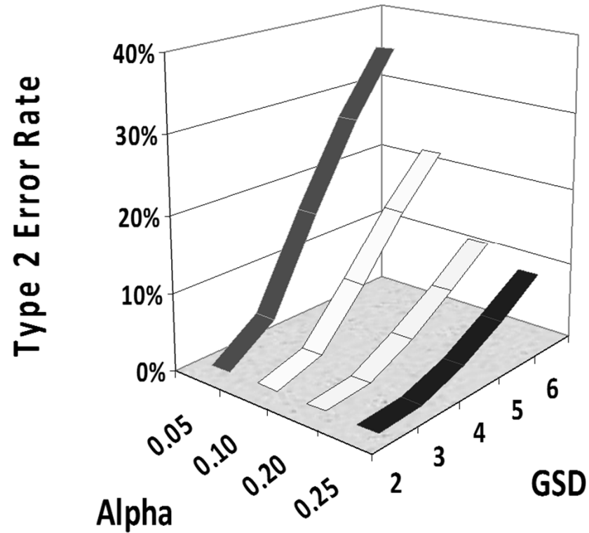
Figure 1. Type 2 Error Rate of WRS Test using 30 Samples from Two Lognormal Distributions: LN(0,1) and LN(1,1)
