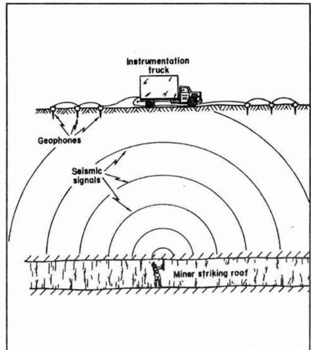
Figure 2.--Trapped miner seismic detection system.
