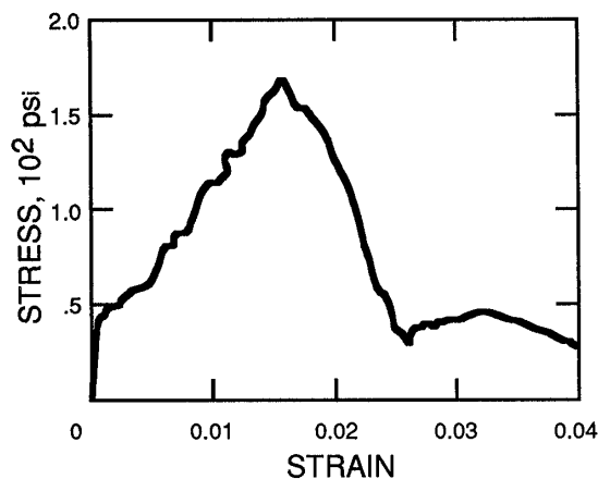
Figure 5.—Numerical model simulation of unconfined compression test with backfill properties.
