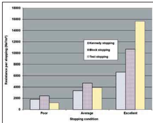
Figure 5. Resistance factors for various stopping types
