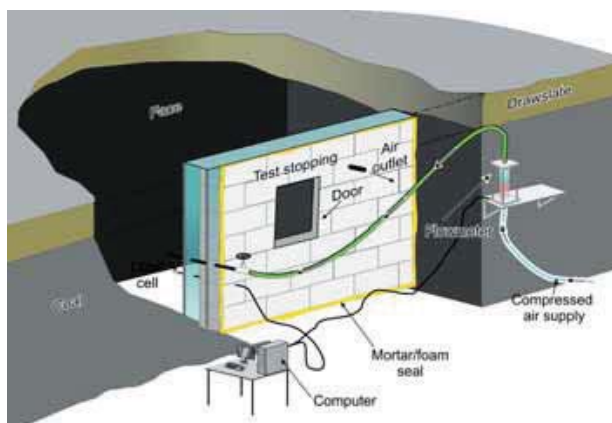
Figure 1. Test setup
