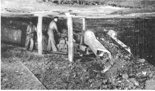
Figure 5. Machine loading with timber support.
