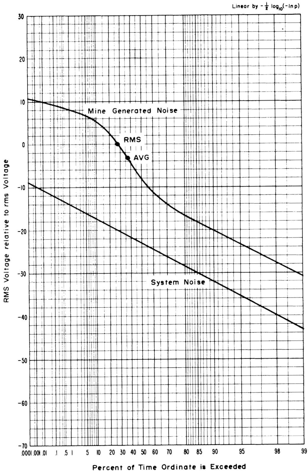
Figure 4-41 APD, 10 kHz, roof bolt measurement, 1.0 kHz predetection bandwidth, April 19, 1973, 1:30 p.m., Farley Headpiece, Itmann #3.
