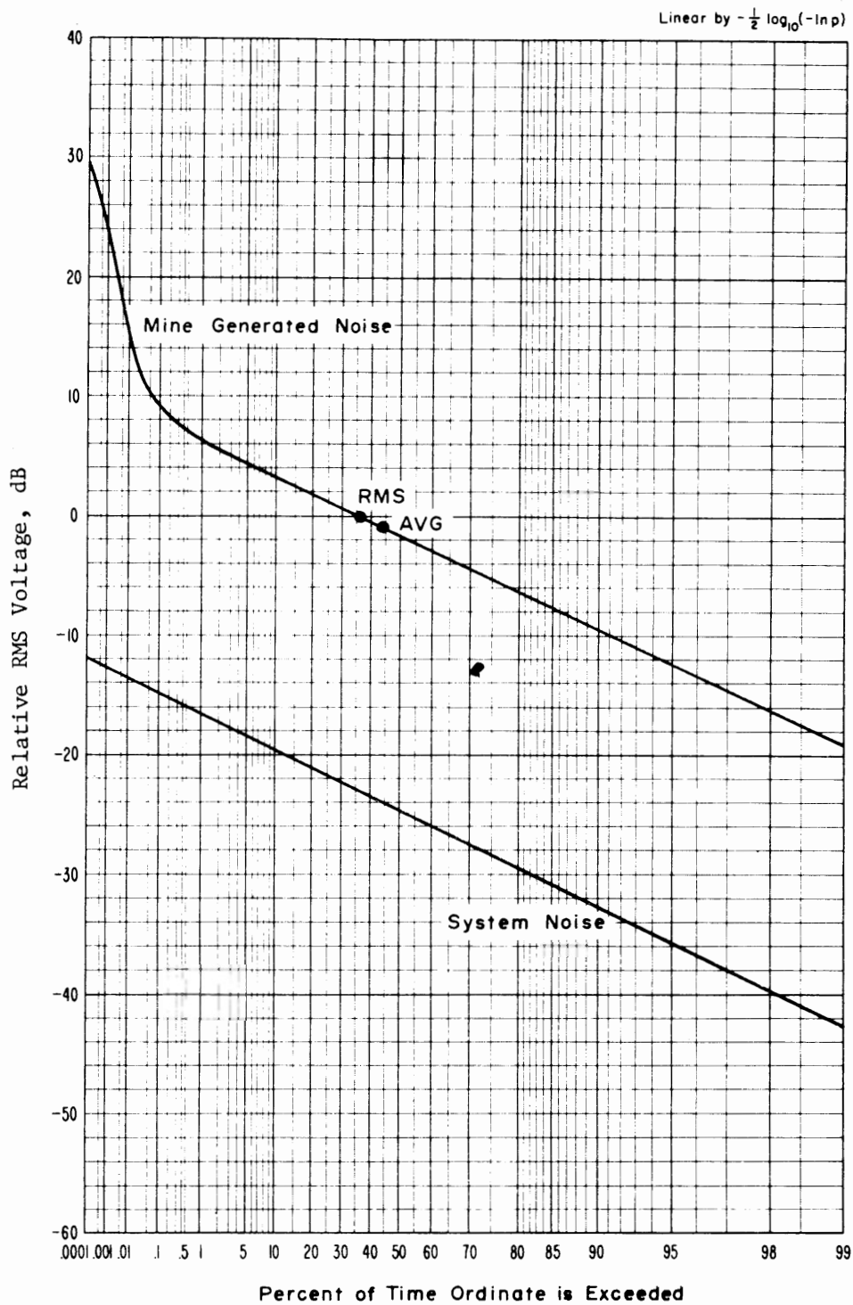
Figure 4-20 APD, 10 kHz, roof bolt measurement, 1.0 kHz predetection bandwidth, April 17, 1973, 5:00 p.m., Cabin Creek, Itmann #3.
