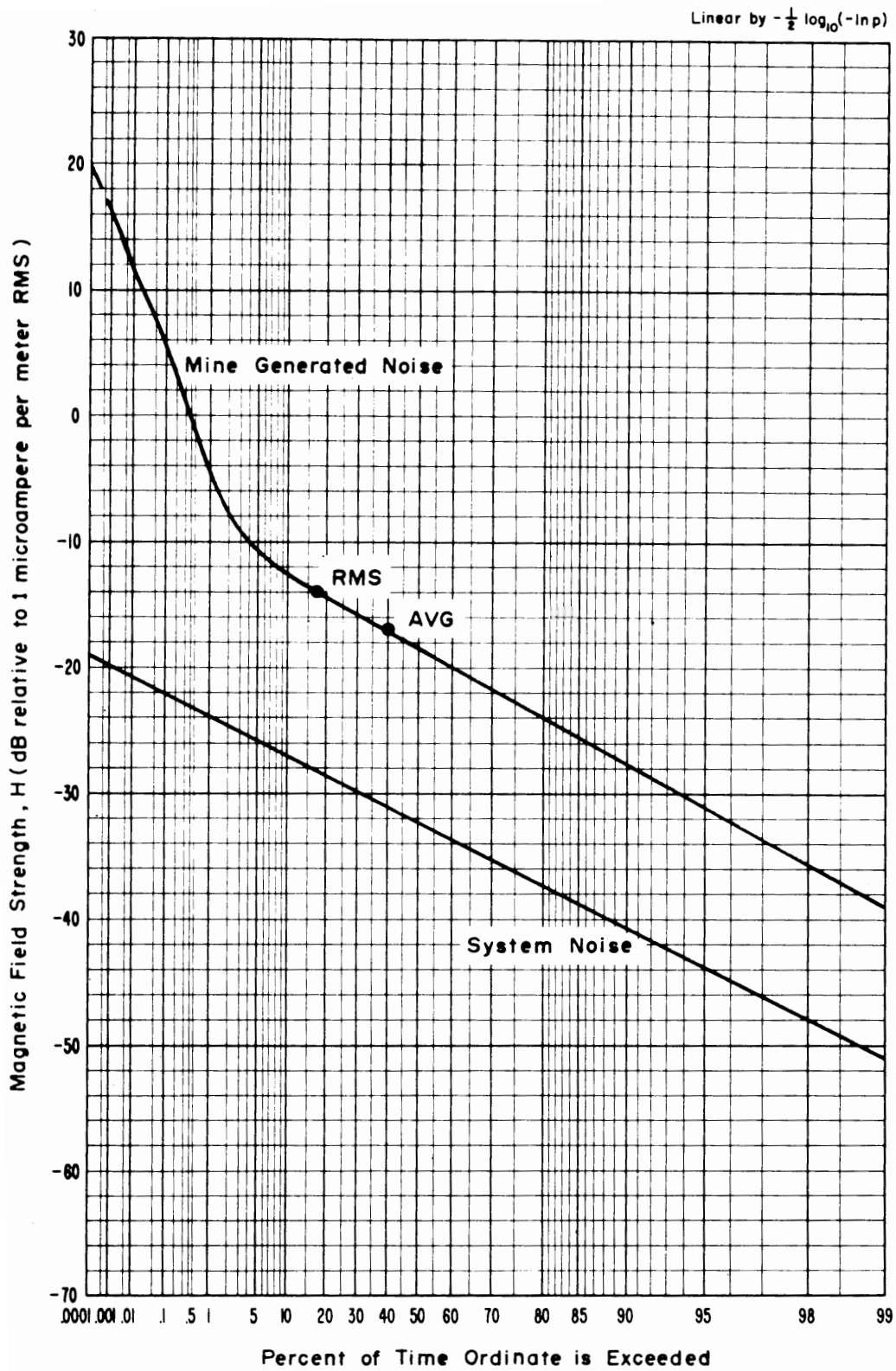
Figure 4-34 APD, 250 kHz, vertical component, 1.0 kHz predetection bandwidth, April 19, 1973, 1:00 p.m., Farley Headpiece, Itmann #3.
