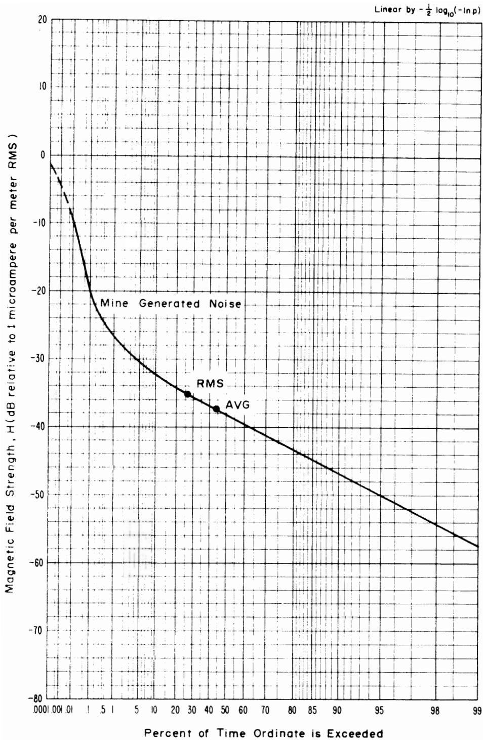
Figure 4-24 APD, 130 kHz, vertical component, 1.0 kHz predetection bandwidth, April 17, 1973, 2:45 p.m., Farley Panel, Itmann #3.
