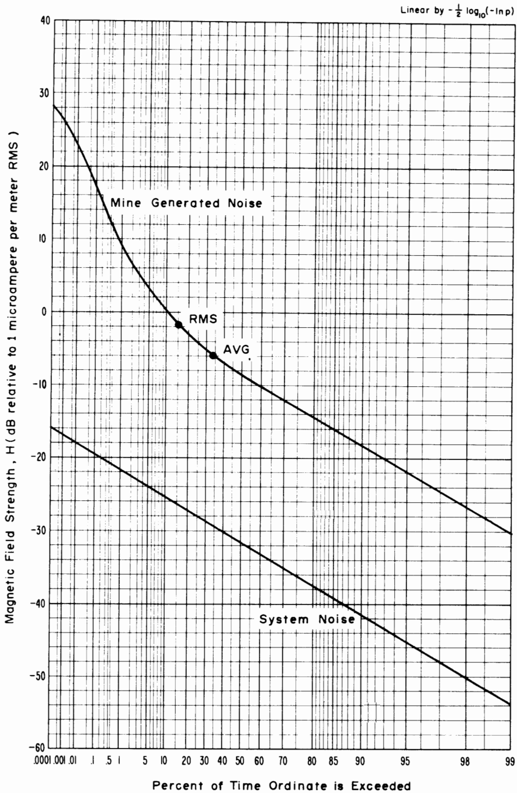
Figure 4-32 APD, 130 kHz, vertical component, 1.0 kHz predetection bandwidth, April 19, 1973, 12:00 p.m., Farley Headpiece, Itmann #3.
