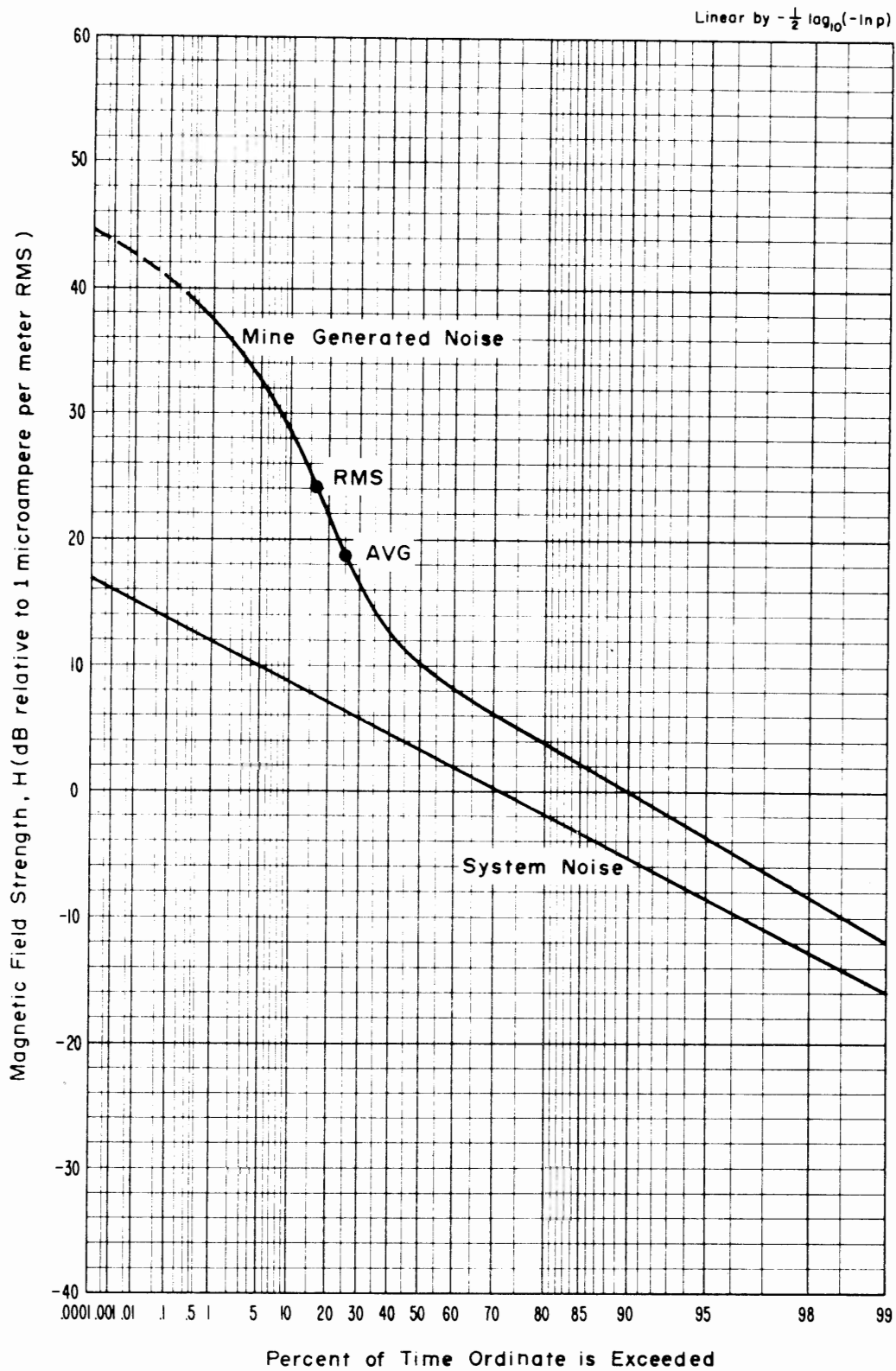
Figure 4-30 APD, 30 kHz, vertical component, 1.0 kHz predetection bandwidth, April 19, 1973, 10:50 a.m., Farley Headpiece, Itmann #3.
