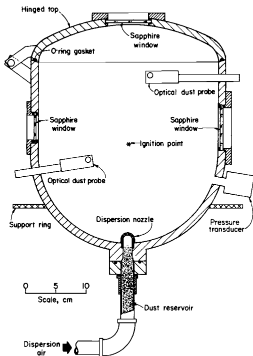
Fig. 4. 20-L laboratory explosibility test chamber.
