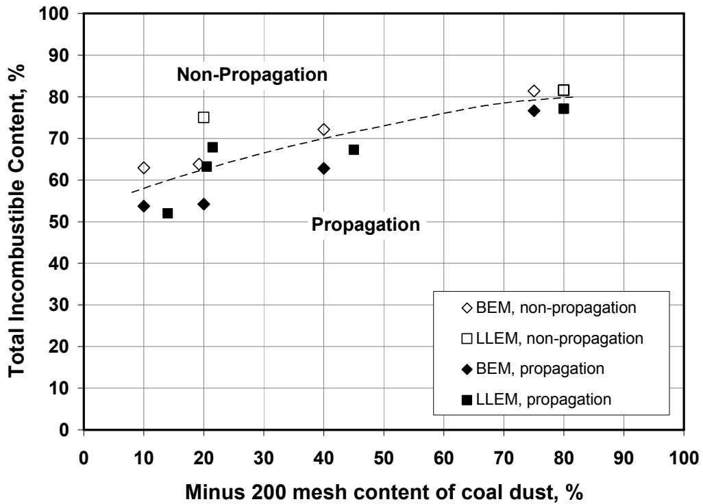
Figure 2. Effect of particle size of coal dust on the explosibility.
