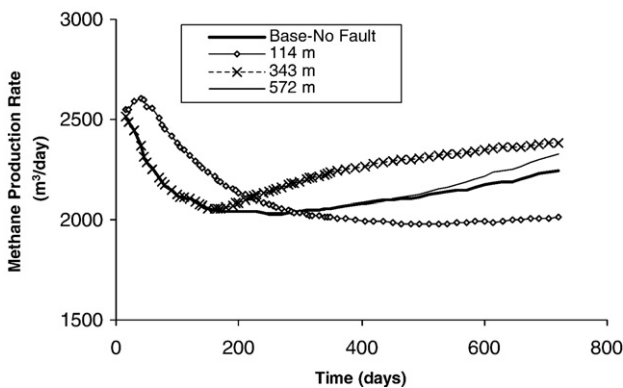
Fig. 6. Methane production curves with a vertical borehole that is located at different distances from an impermeable fault.
