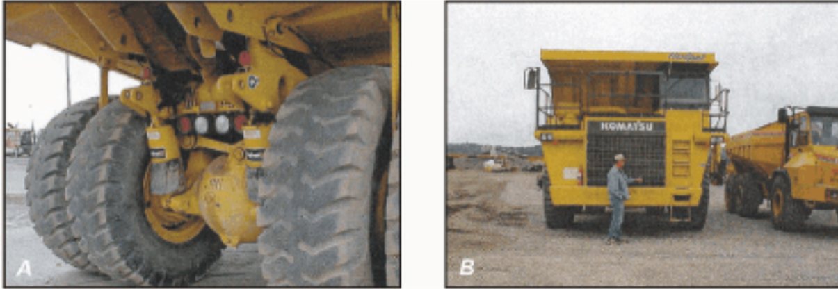
Figure A-3.—Mounting positions for RFID sensors.
