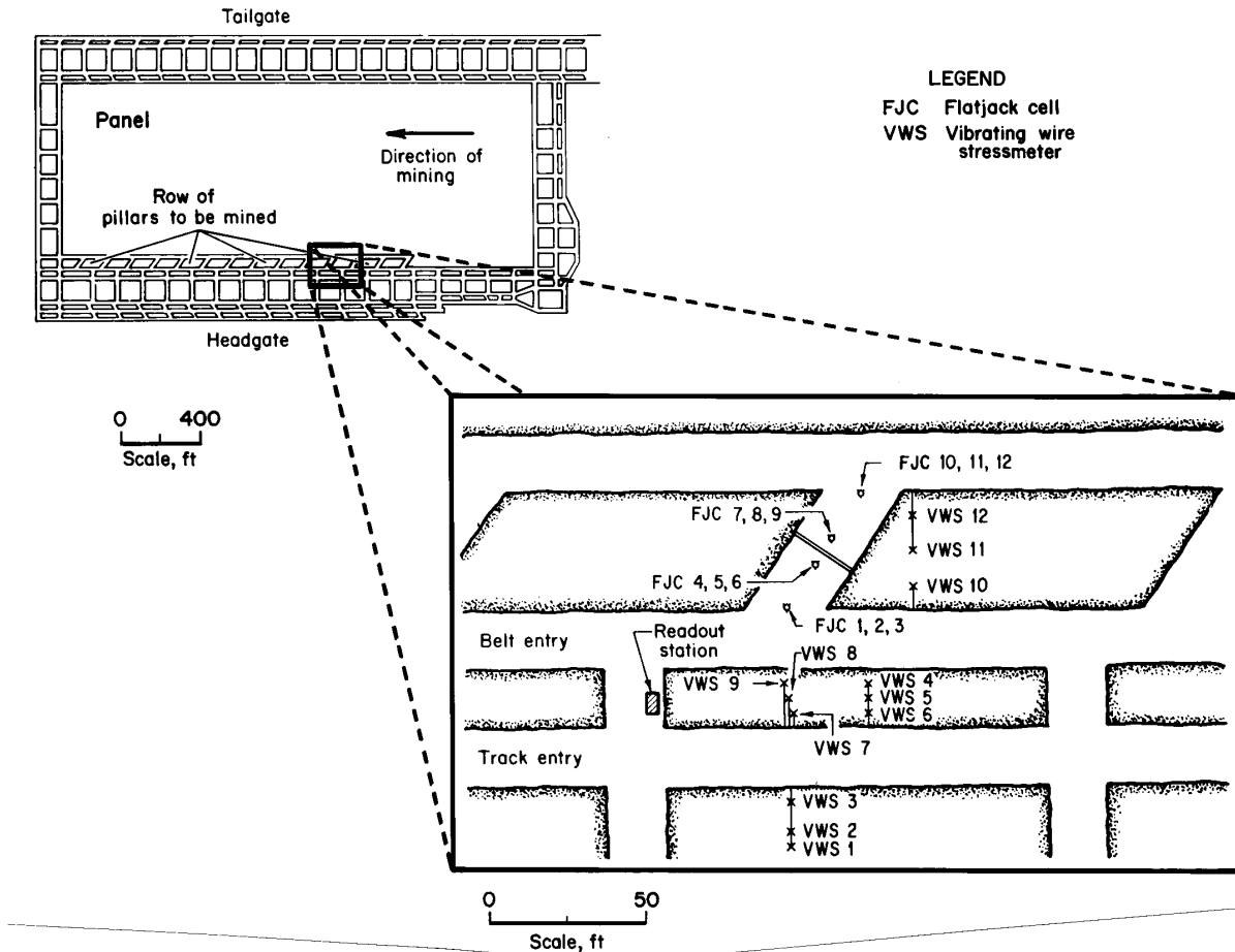
Figure 6.—Detailed area of instrumentation site.
