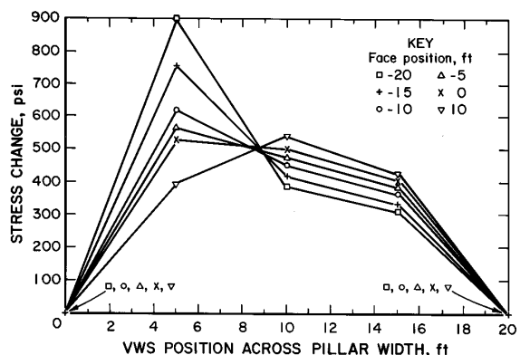
Figure 12.—Stress profile across pillar P2.
