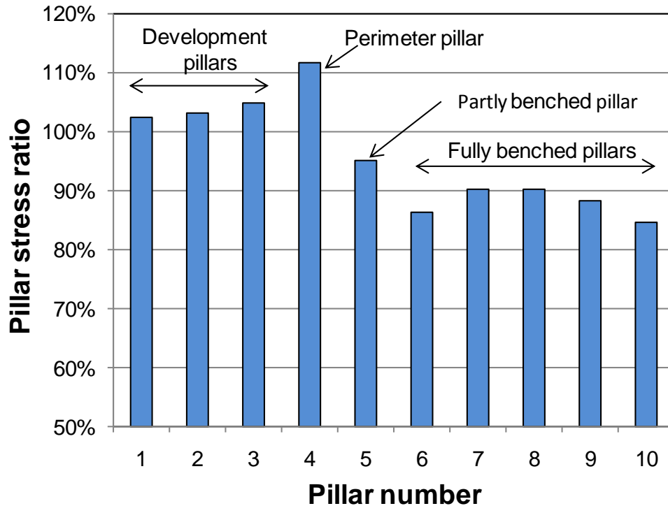
Figure 22. Results of numerical model showing the average pillar stress during bench mining as a ratio of the average pillar stress prior to bench mining.
