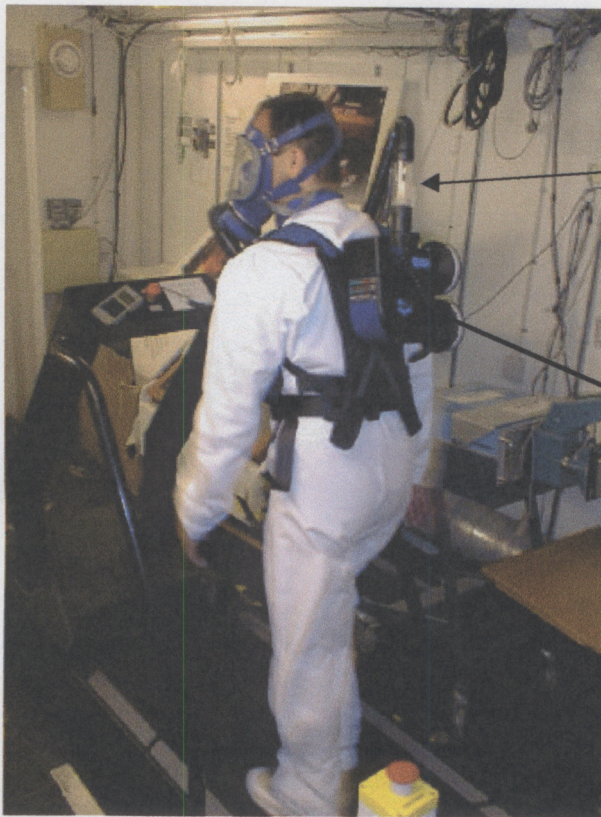
Figure 2. Experimental setup in climatic chamber with treadmill for graded exercise levels. Fan and filter are worn in a separate house on the back. Full face mask is connected to the house via a flexible tube. At the tube end nearest to the house a separate flow meter was mounted.
