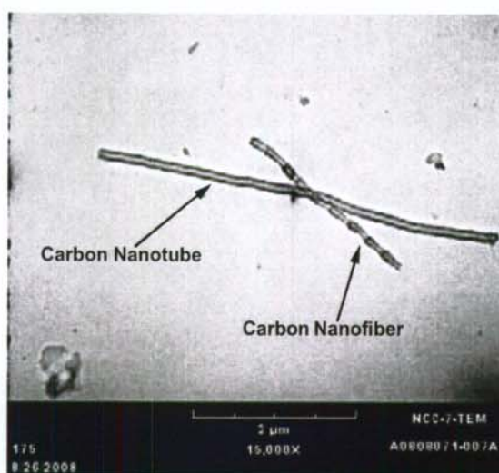
Figure 4. Electron microscopy micrograph of a carbon nanofiber and carbon nanotube
