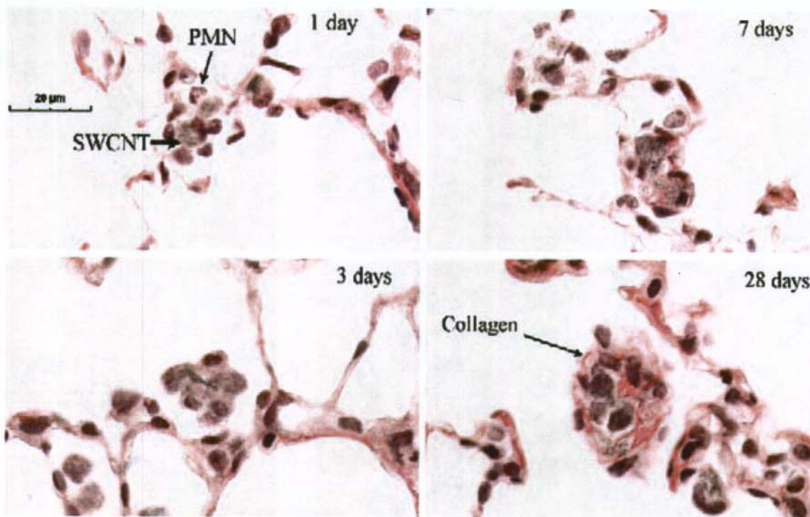
Figure 5-1. Formation of collagen following deposition of SWCNTs in the lungs of mice
