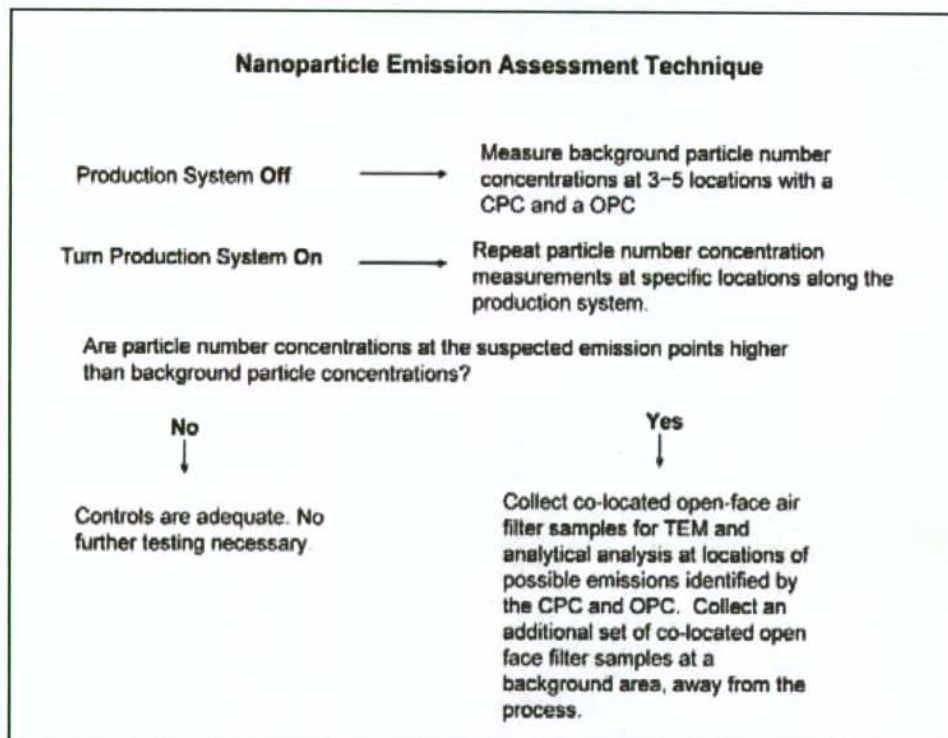
Figure 2. Summary of the initial assessment technique
