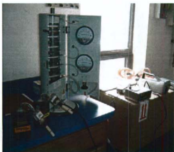
Figure 7-1. Examples of different sampling instruments used to measure occupational exposures to nanoparticles including the determination of real-time particle number concentrations and size-fractionated mass concentrations
