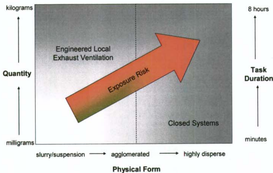
Figure 8–3. Factors influencing control selection. Several factors influence the selection of exposure controls for nanomaterials including quantity of nanomaterial handled or produced, physical form, and task duration. As each one of these variables increase, exposure risk becomes greater as does the need for more efficient exposure control measures.
