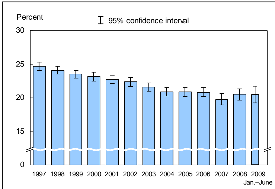
Figure 8.1. Prevalence of current smoking among adults aged 18 years and over: United States, 1997-June 2009
