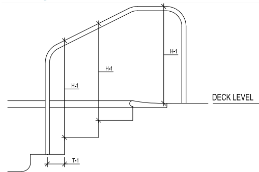
Figure 4.5.5.7.1: Stair Handrails: Side View
