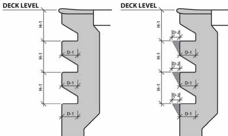
Figure 4.5.7.4.2: Recessed Step Dimensions: Front View
